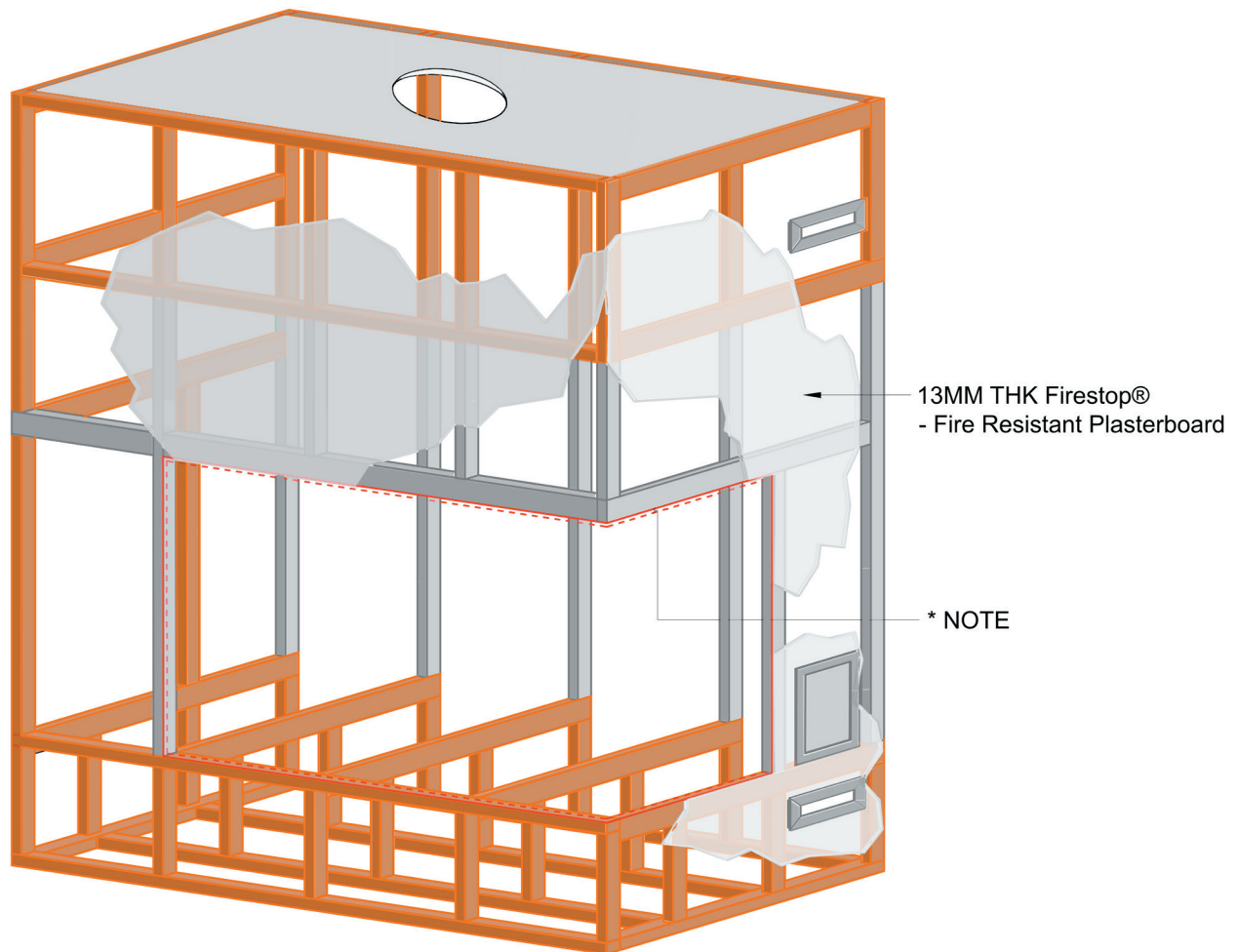
Figure 1.7 (Cladding Material)
