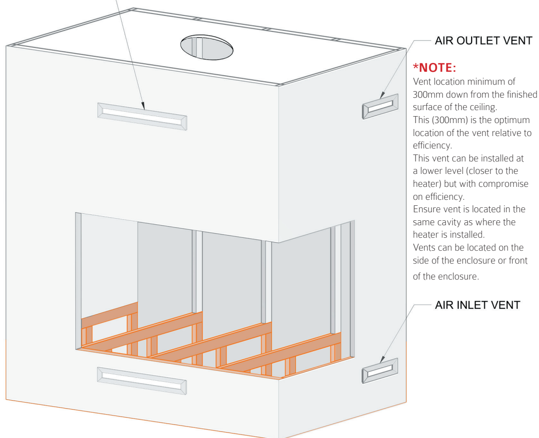
Figure 1.2 (Vents)
