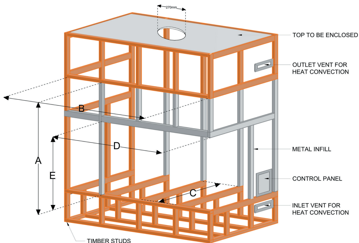
Figure 1.8 (Timber framing)
